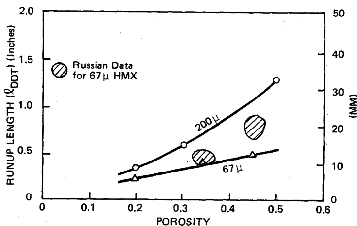
Fig 5 Variation of runup length with porosity (Ref 17)
